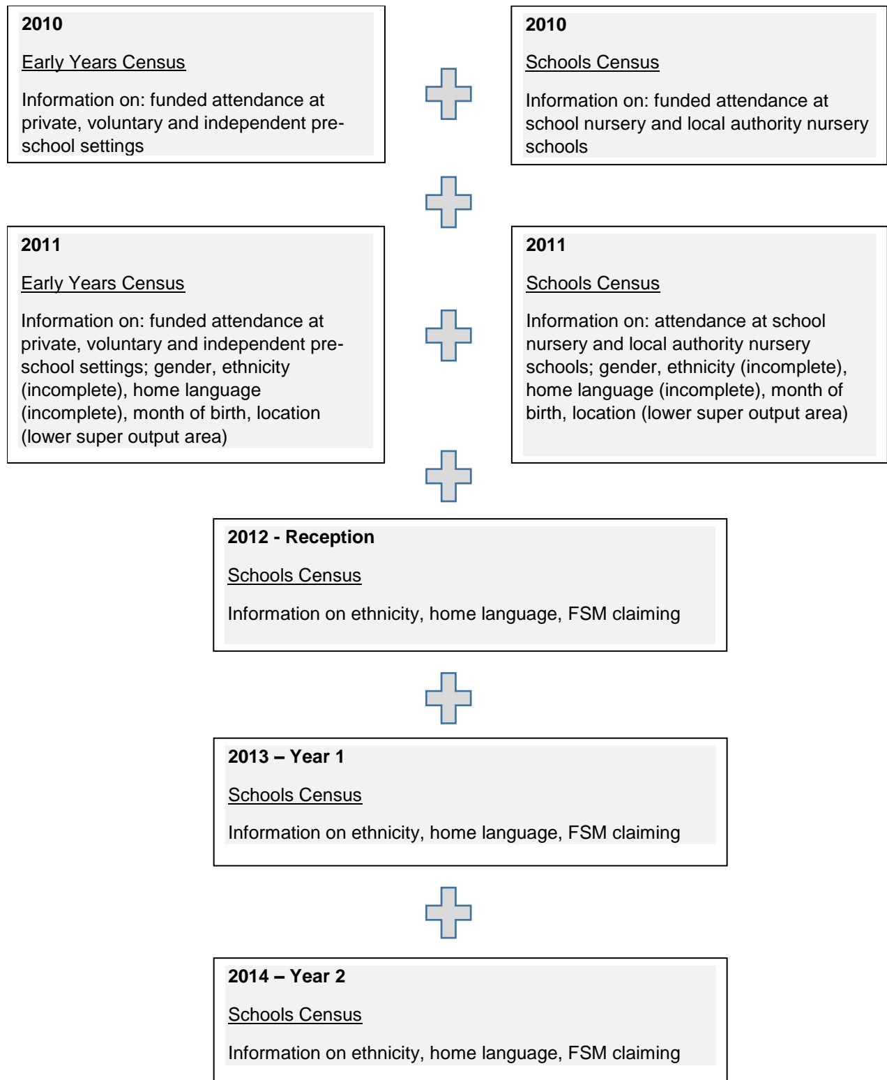
Figure 1: Data structure
